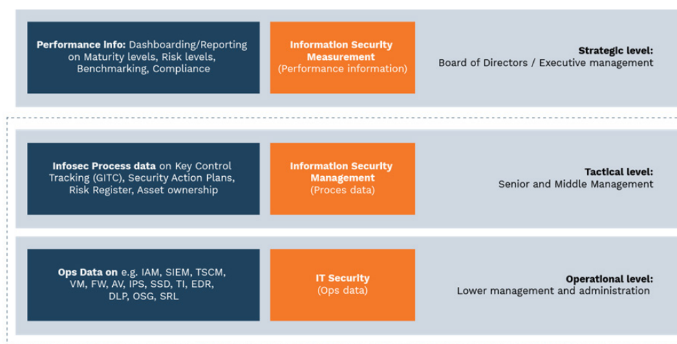
Figure 2: Conceptual model with detailed BIS processes and data, based on Von Solms and Von Solms [23].
