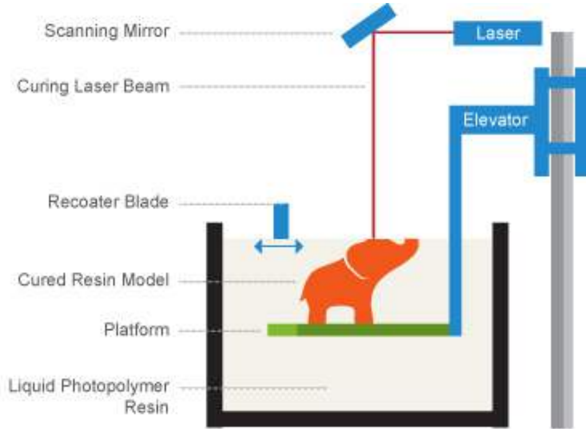
Stereolithography
